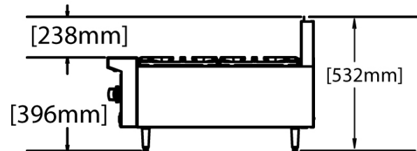
Modular Top Side View w/4" [102mm] Adj. Legs
